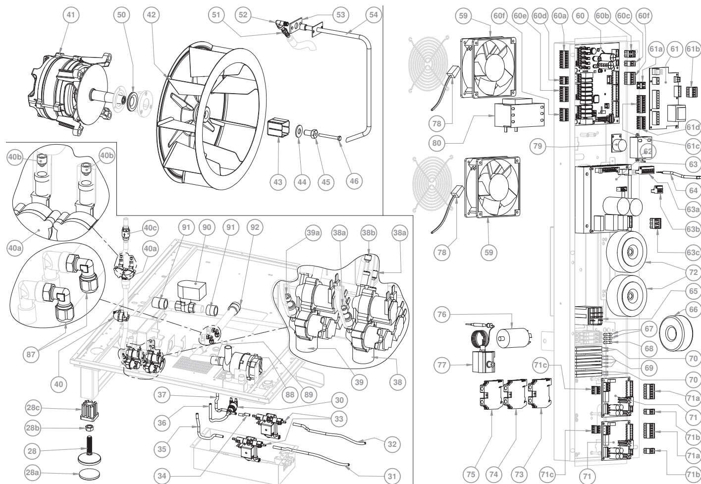
Exploded view 2/4
