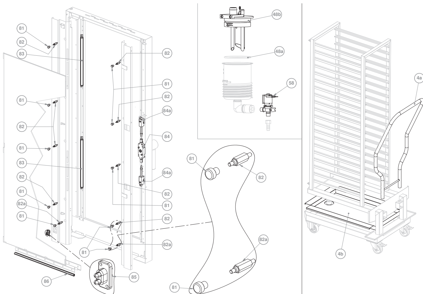
Exploded view 3/4
